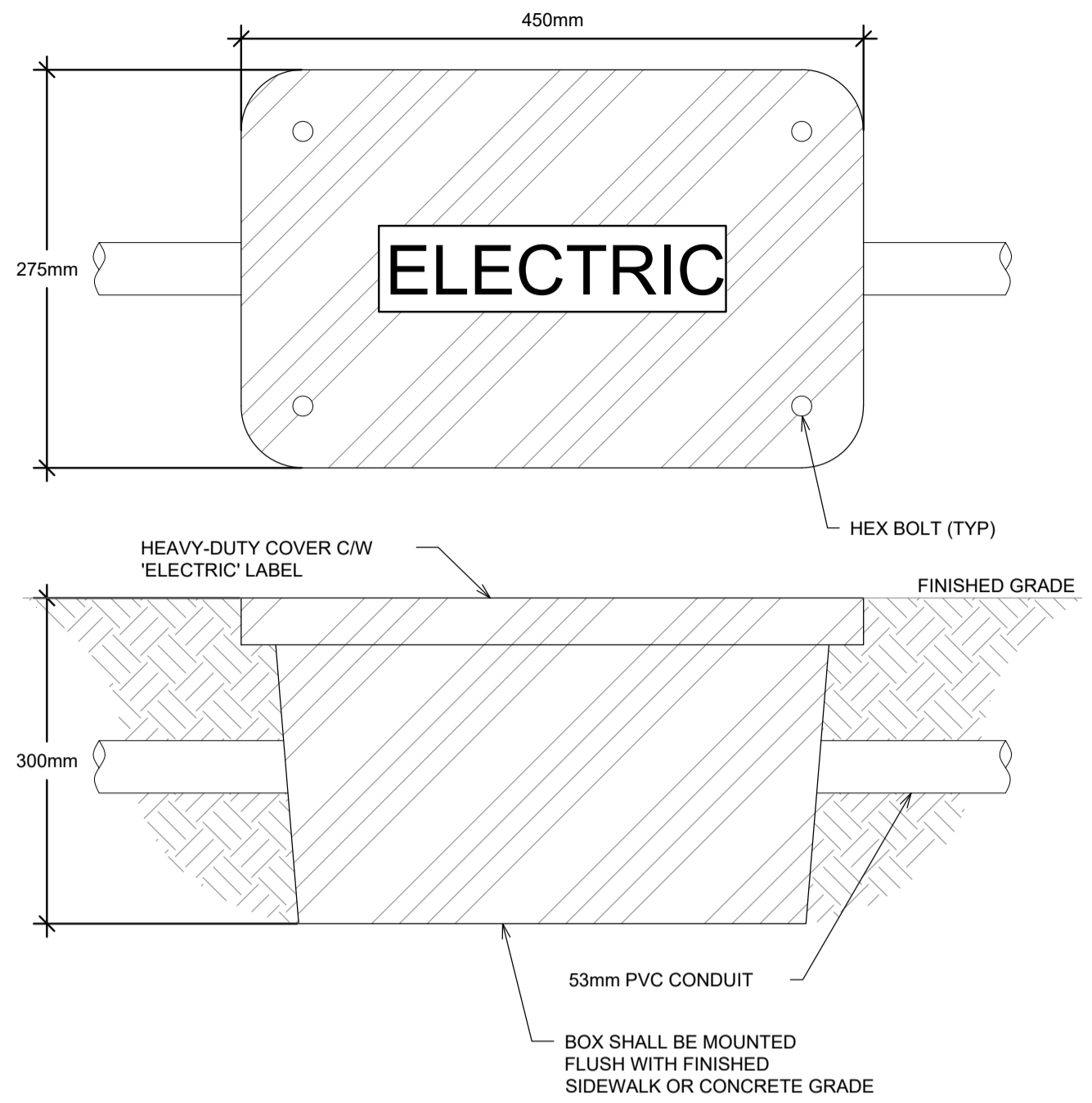
2 HEAVY DUTY BELOW GRADE PULLBOX E1.0 N.T.S.
